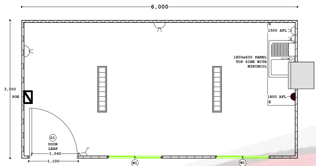
3 FLOOR PLAN 1:50
