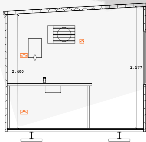
7 CROSS SECTION 1:50
