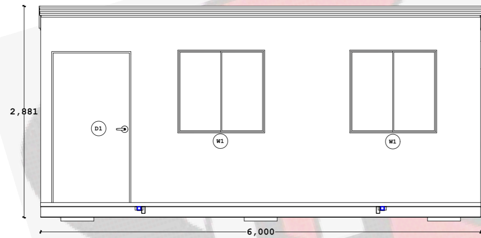
5 FRONT ELEVATION VIEW 1:50
