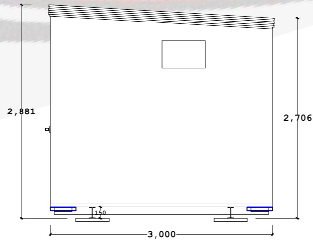
6 RIGHT ELEVATION VIEW 1:50
