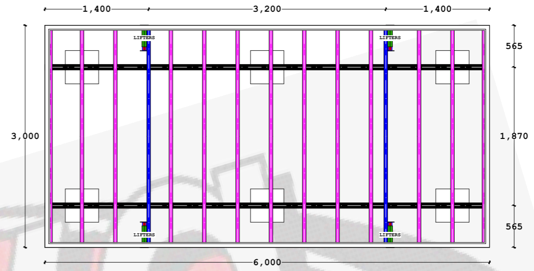
4 BASE FRAME VIEW 1:50
