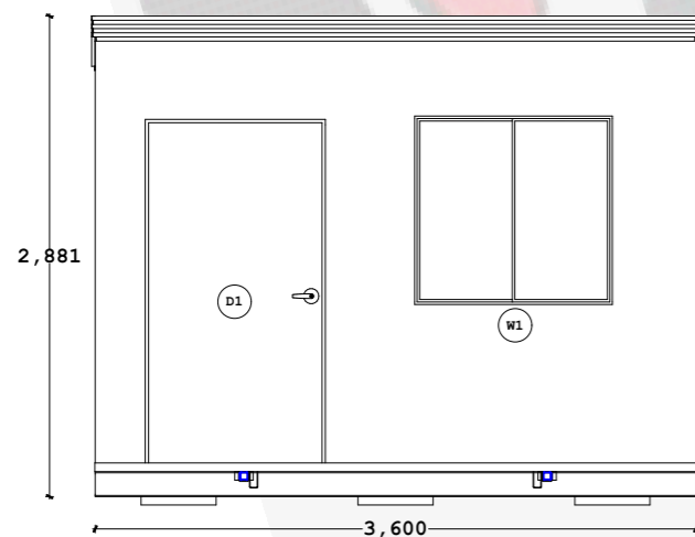
5 FRONT ELEVATION VIEW 1:50
