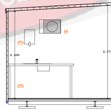
7 CROSS SECTION 1:50
