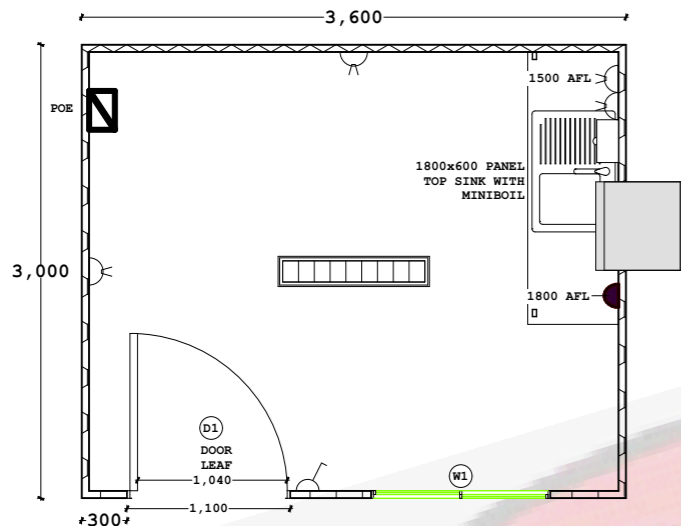
3 FLOOR PLAN VIEW 1:50
