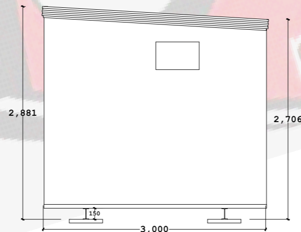
6 SIDE ELEVATION VIEW 1:50
