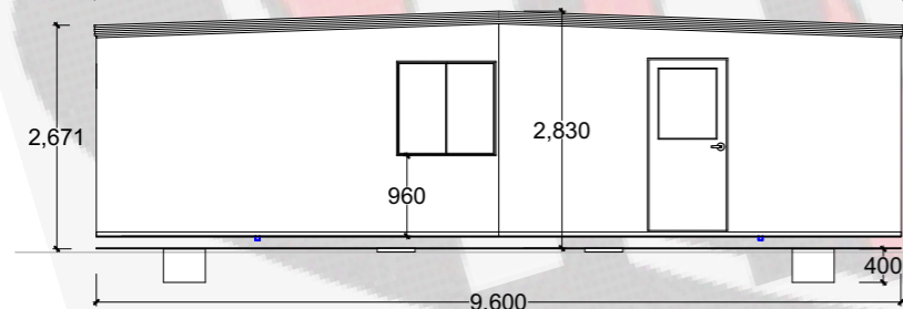
4 REAR ELEVATION 1:100
