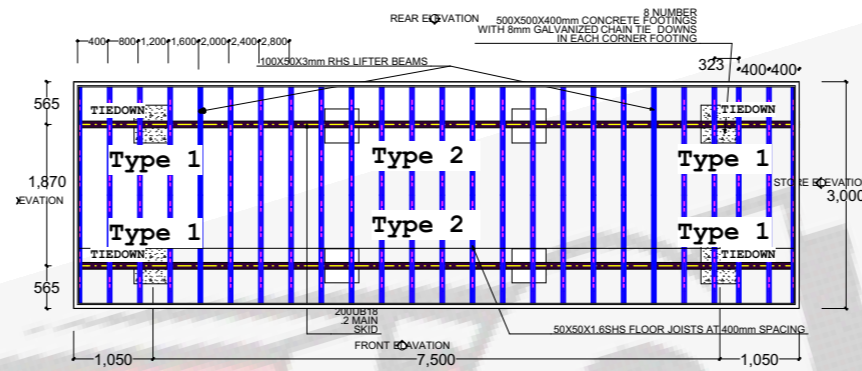
2 BASE FRAME 1:100
