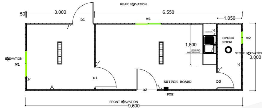
1 floor plan 1:100
