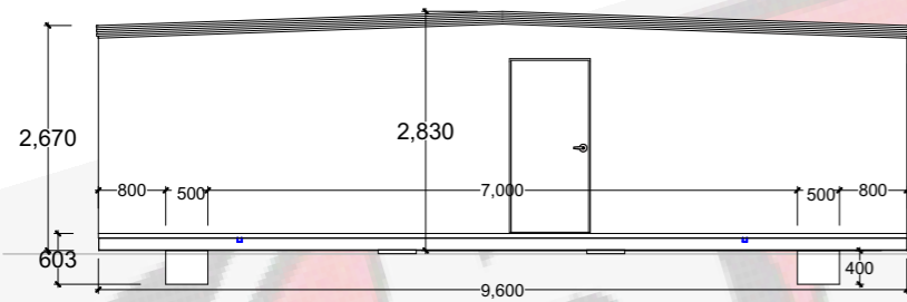
3 FRONT ELEVATION 1:100
