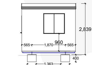
5 OFFICE ELEVATION 1:100
