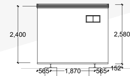
6 STORE ELEVATION 1:100
