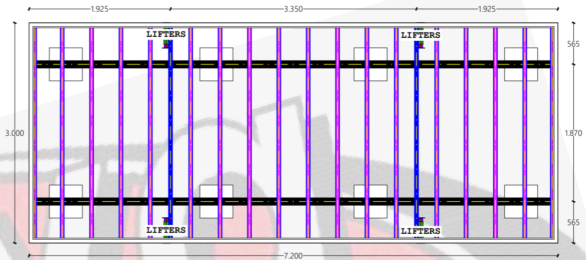
3 BASE FRAME VIEW 1:50
