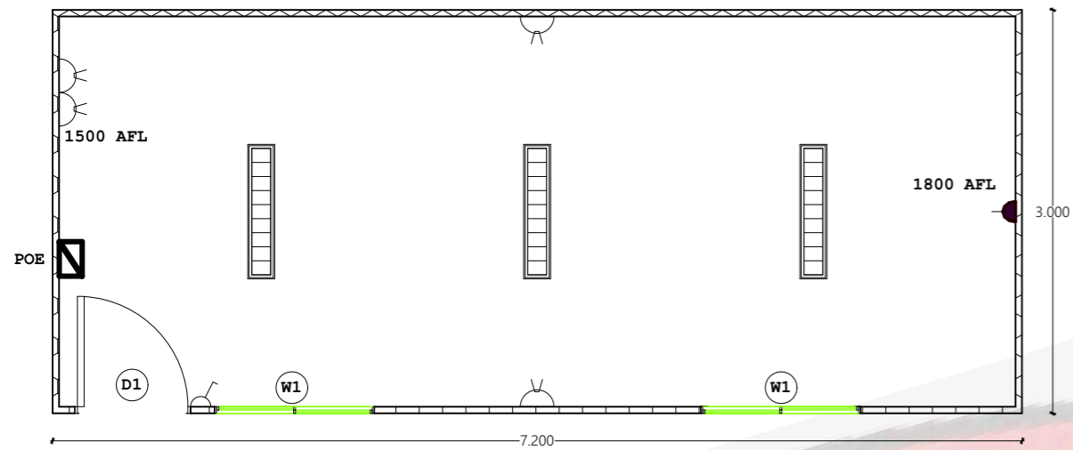
1 FLOOR PLAN VIEW 1:50
