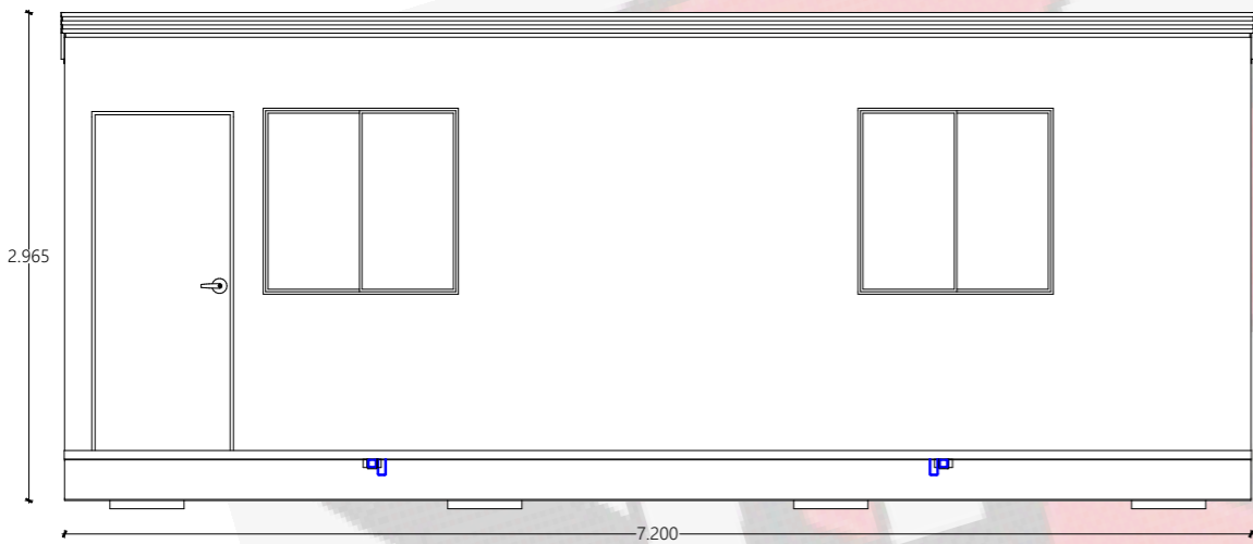
2 FRONT ELEVATION VIEW 1:50
