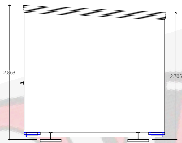
2 SIDE ELEVATION VIEW 1:50
