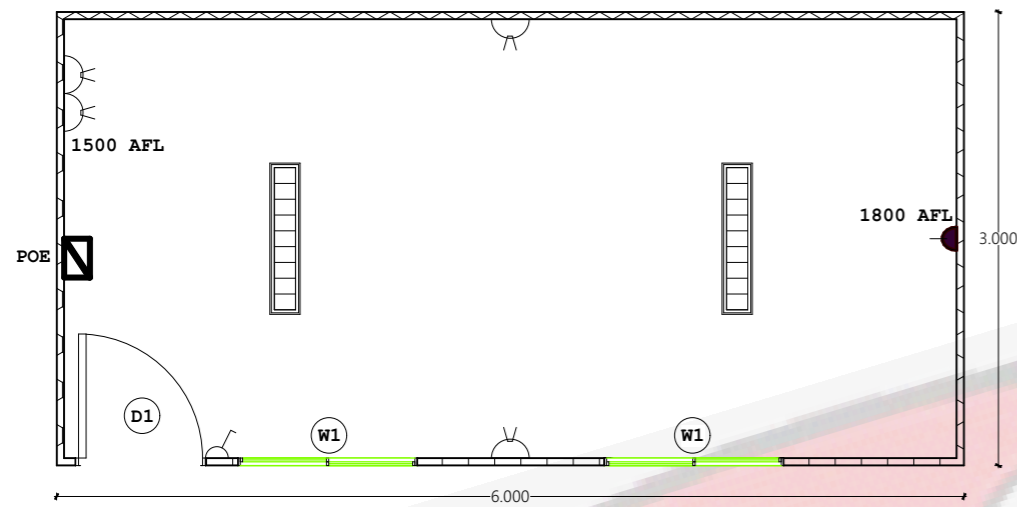
1 FLOOR PLAN VIEW 1:50
