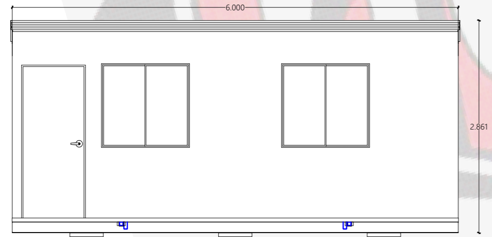
3 FRONT ELEVATION VIEW 1:50
