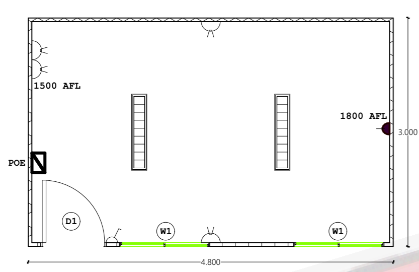
1 FLOOR PLAN VIEW 1:50
