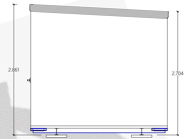
4 SIDE ELEVATION VIEW 1:50
