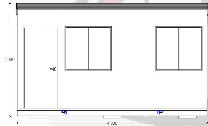
2 FRONT ELEVATION VIEW 1:50
