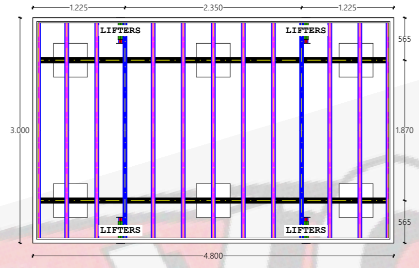
3 BASE FRAME VIEW 1:50
