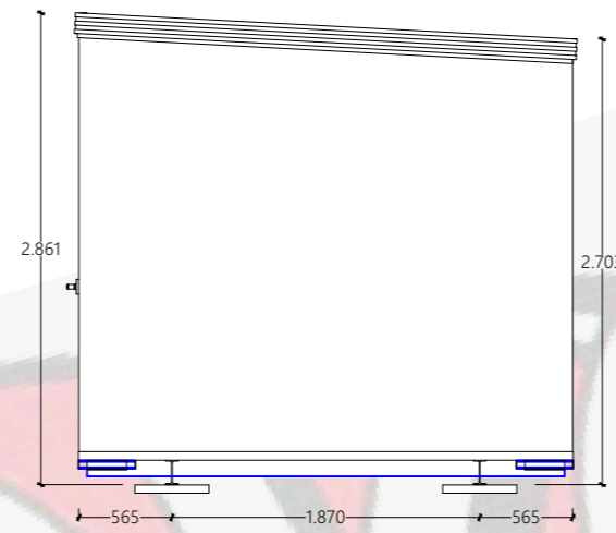
3 SIDE ELEVATION VIEW 1:50
