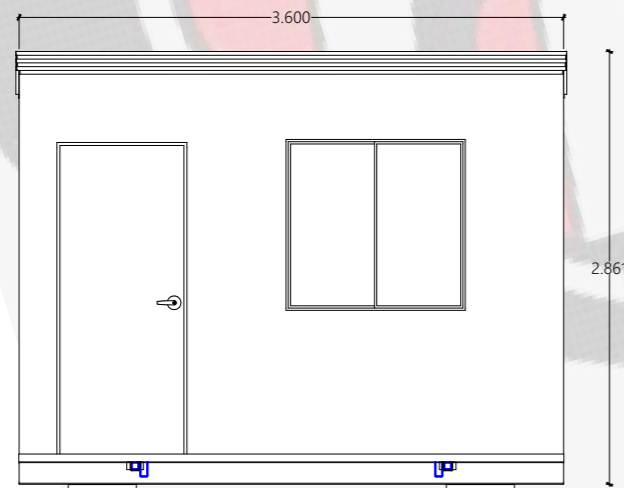
2 FRONT ELEVATION VIEW 1:50
