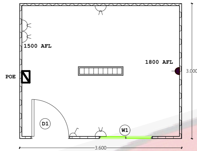
1 FLOOR PLAN VIEW 1:50
