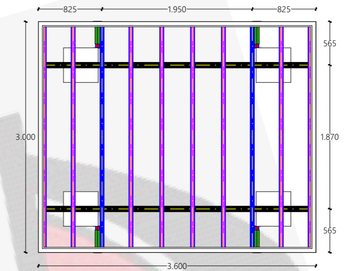
4 BASE FRAME VIEW 1:50
