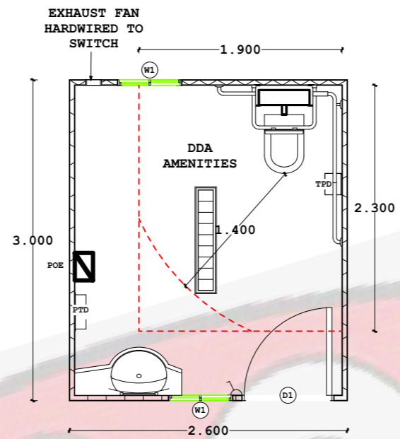
3 FLOOR PLAN VIEW 1:50
