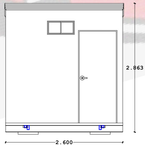
6 FRONT ELEVATION VIEW 1:50
