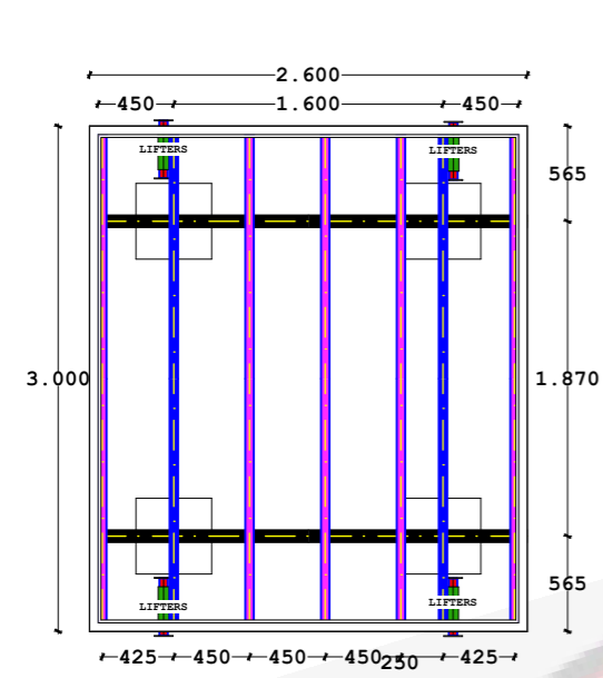
4 BASE FRAME VIEW 1:50
