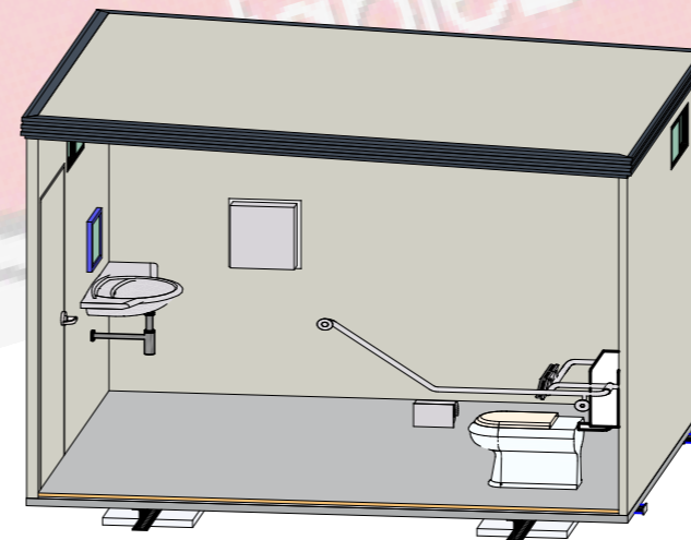
9 3D INTERIOR 1:50
