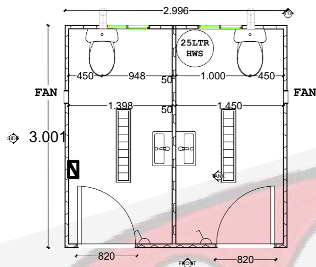
1 FINISH FLOOR 1:50
