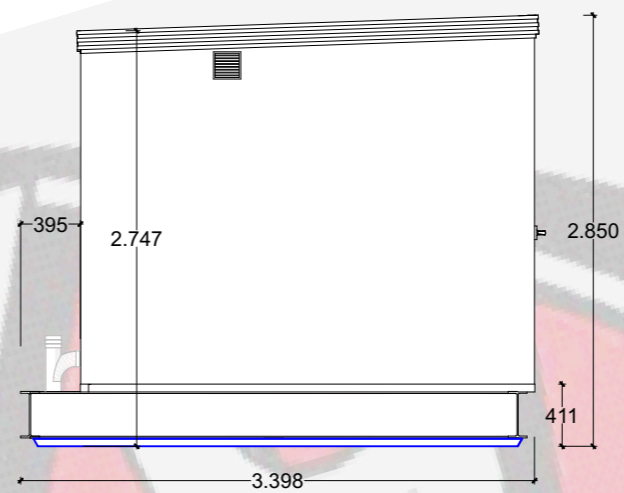
3 SIDE VIEW 1:50
