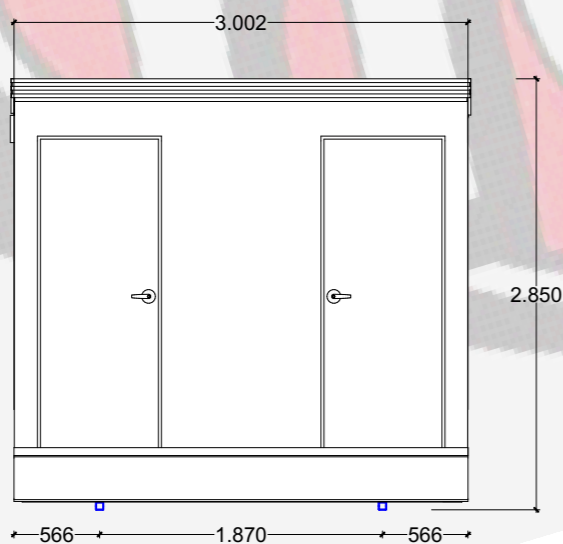
2 FRONT VIEW 1:50
